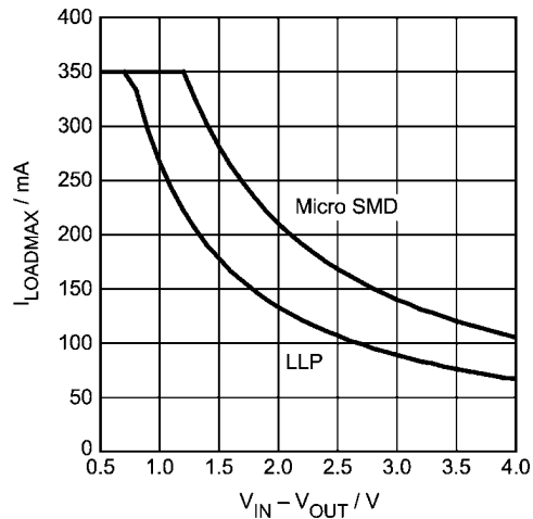
FIGURE 3. Maximum Load Current vs V_{IN} - V_{OUT} , T_A = 85^\circ\text{C} , V_{OUT} = 1.5\text{V} , \theta_{JA(MICROSMD)} = 95^\circ\text{C/W} , \theta_{JA(LLP)} = 150^\circ\text{C/W} ,
